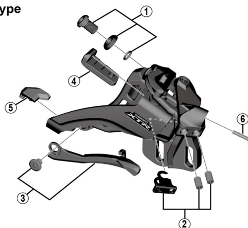
High clamp
