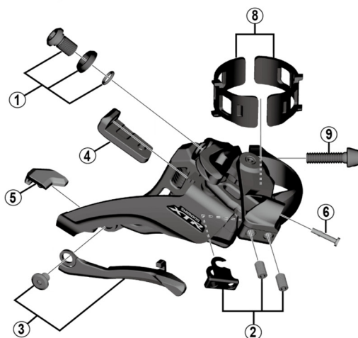
Low clamp
