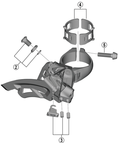
Middle clamp
